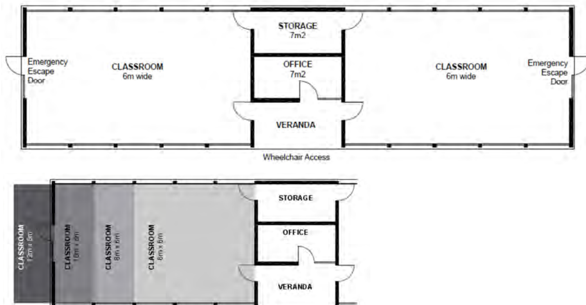
Figure 3: Hybrid Building Floor Plan (Source: Kaunitz 2011)
